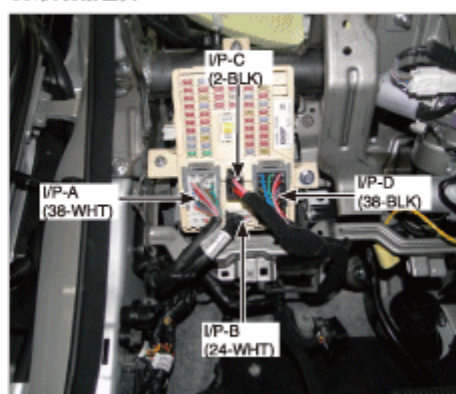
59.仪表板左侧
