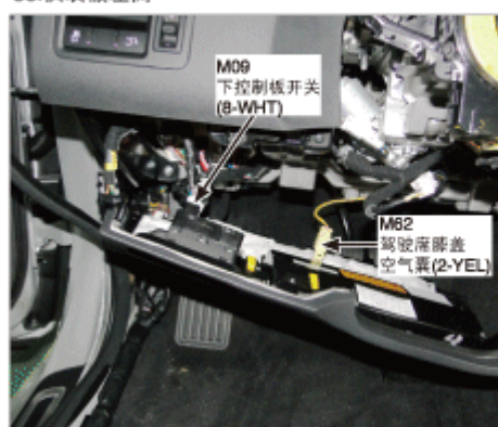
58.仪表板左侧
